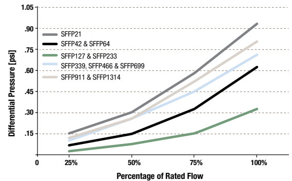
SFFP Dry Particulate Filter Initial Dry Differential Pressure (25% - 100% Rated Flow)
