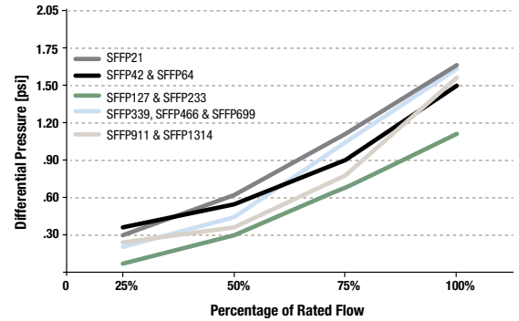
SFFP Coalescing Filter Initial Saturated Differential Pressure (25% - 100% Rated Flow) ISO12500-1 Challenge - 10mg/m 3
